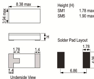
Outline (mm) -SM1 = Gold plated (RoHS)
